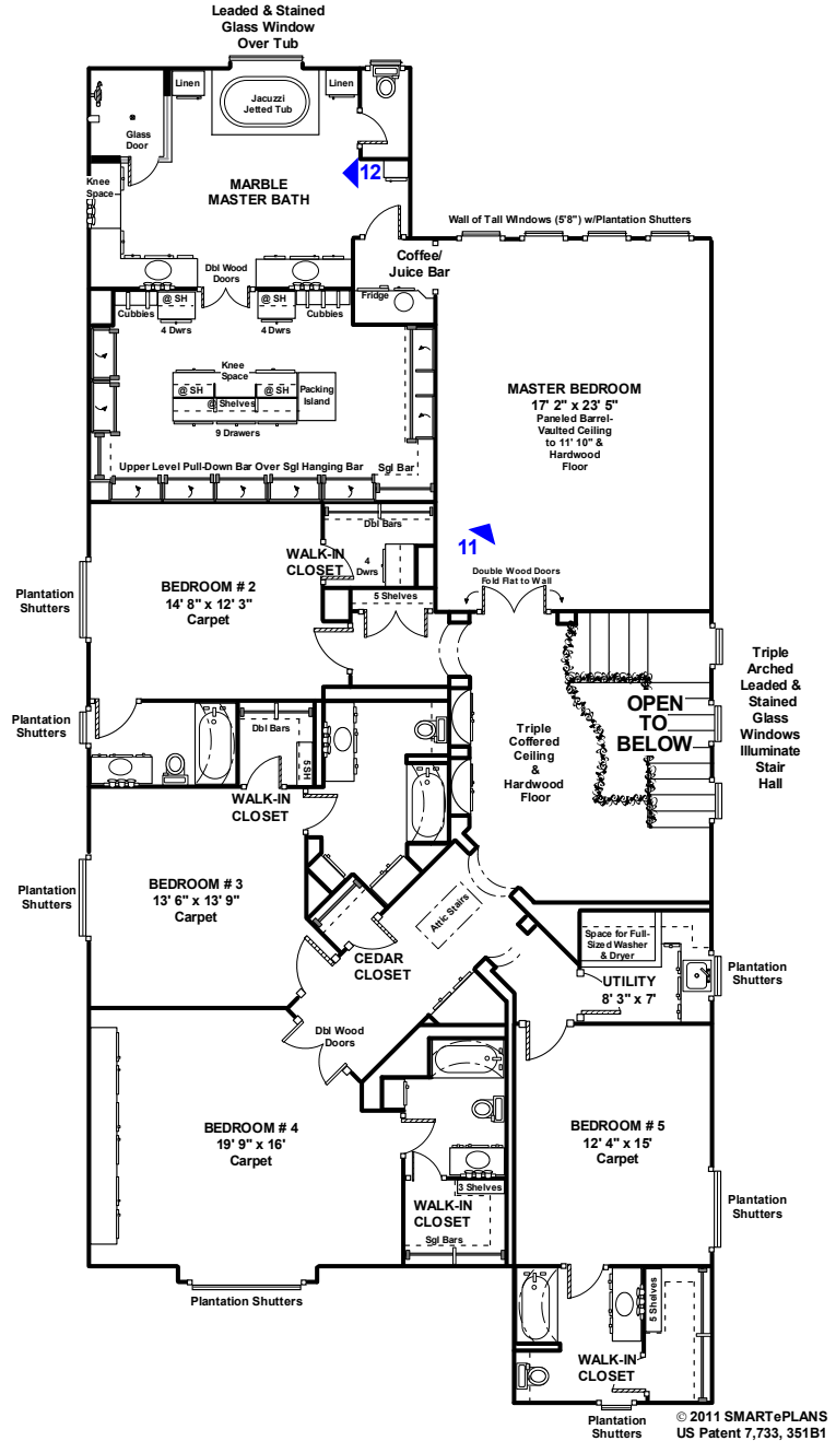
SECOND FLOOR
